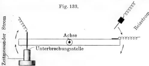
Helmholtz'sche Wippe.
